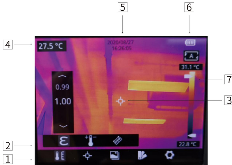
Figure8.4 User Interface
